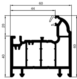
60mm Outer Frame
