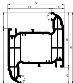
88mm Z Transom
