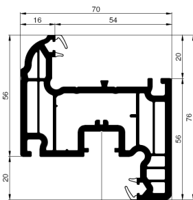
76mm Tilt N Turn Sash
