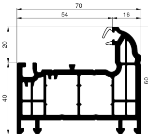
60mm Outer Frame
