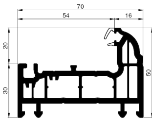
50mm Outer Frame
