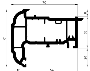
61mm Dummy Mullion
