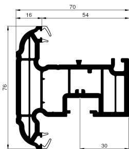
76mm T Sash
