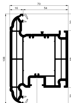
108mm T Sash
