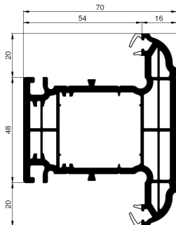
88mm T Transom
