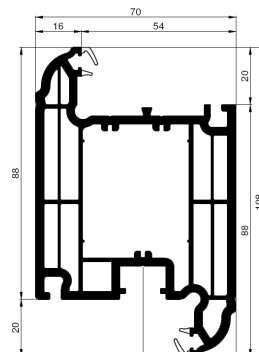
108mm Z Sash
